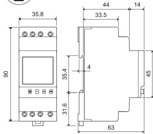
12.51/12.81 Screw terminal
